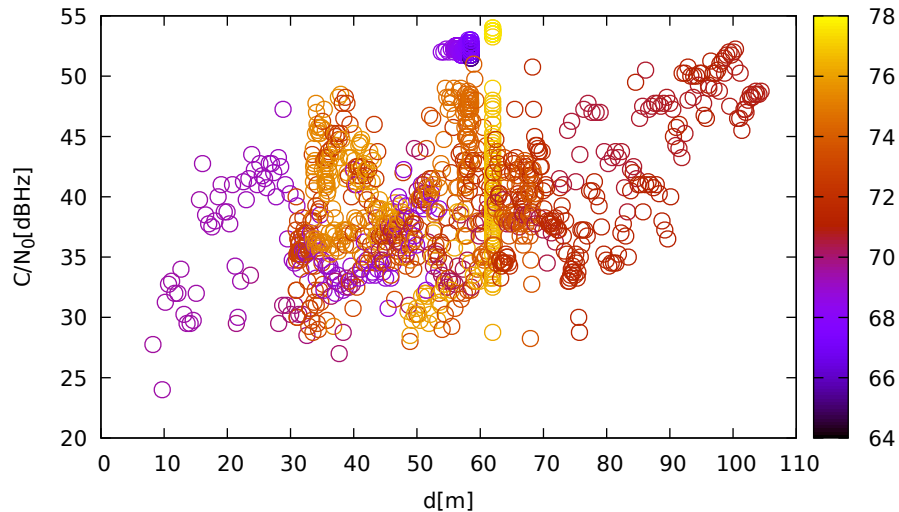
C/N 0 vs distance (LeicaGS18 at C 1 for G01 at L1)
