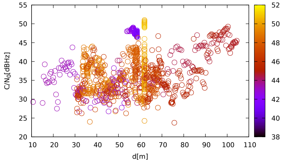
C/N 0 vs distance (LeicaGS18 at C 1 for G03 at L1)
