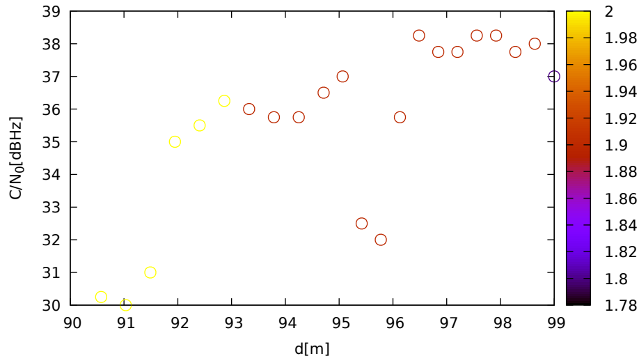
C/N 0 vs distance (LeicaGS18 at C 1 for G04 at L1)
