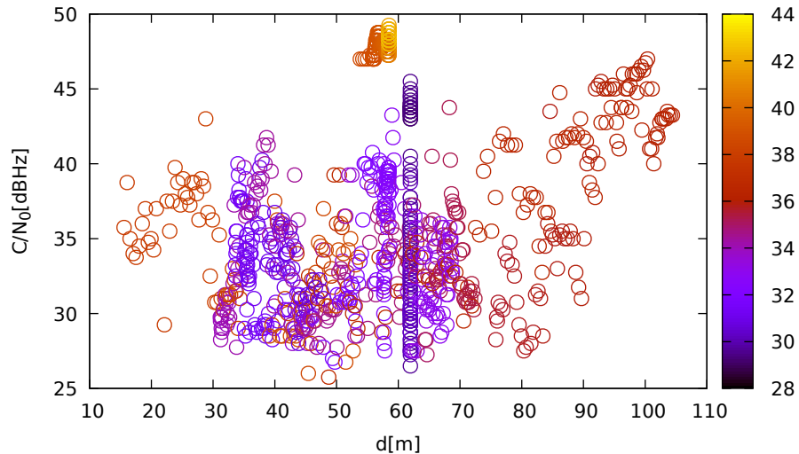
C/N 0 vs distance (LeicaGS18 at C 1 for G08 at L1)
