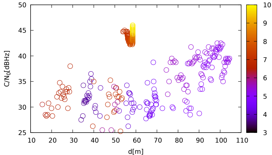
C/N 0 vs distance (LeicaGS18 at C 1 for G10 at L1)
