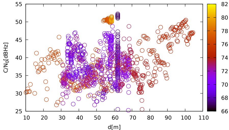
C/N 0 vs distance (LeicaGS18 at C 1 for G11 at L1)
