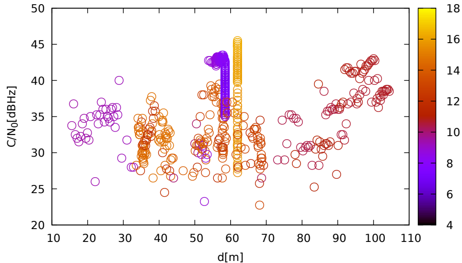
C/N 0 vs distance (LeicaGS18 at C 1 for G17 at L1)
