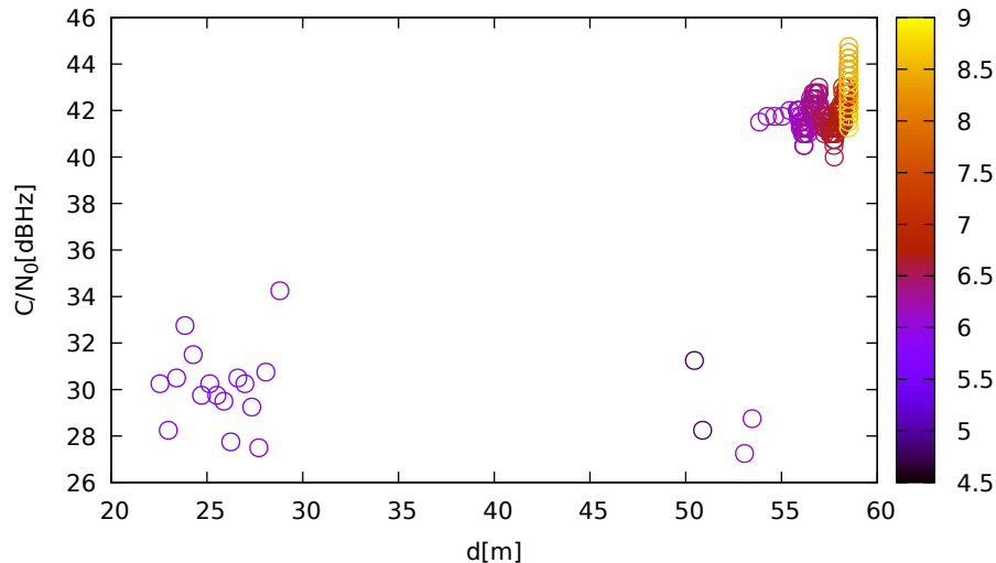
C/N 0 vs distance (LeicaGS18 at C 1 for G21 at L1)
