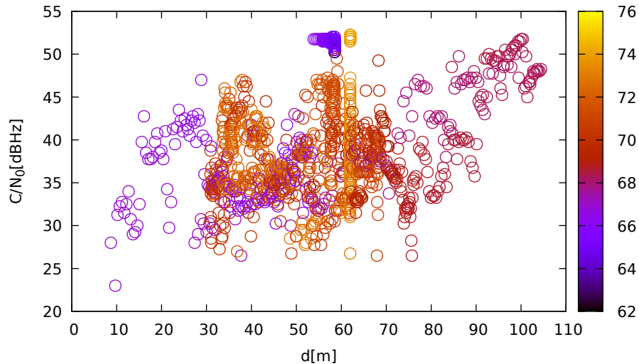
C/N 0 vs distance (LeicaGS18 at C 1 for G22 at L1)
