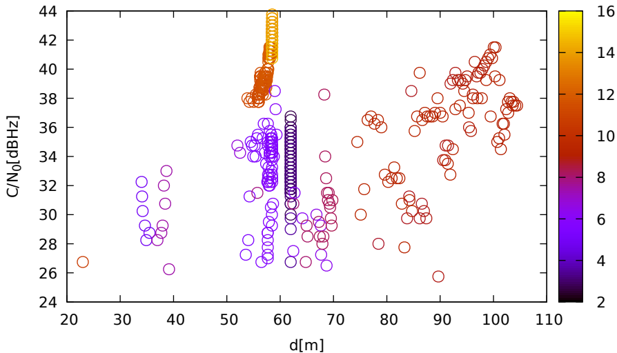
C/N 0 vs distance (LeicaGS18 at C 1 for G27 at L1)
