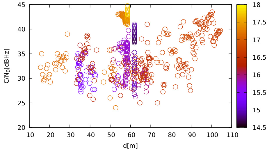
C/N 0 vs distance (LeicaGS18 at C 1 for G28 at L1)
