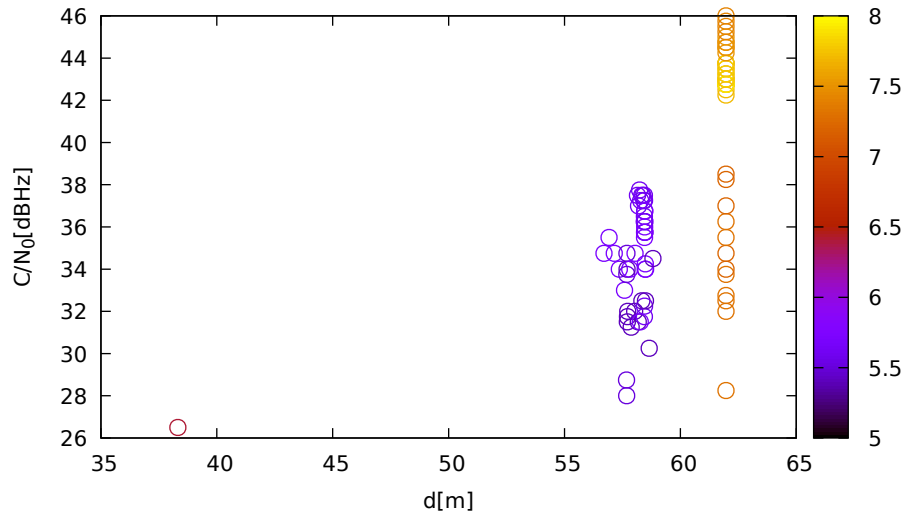
C/N 0 vs distance (LeicaGS18 at C 1 for G31 at L1)
