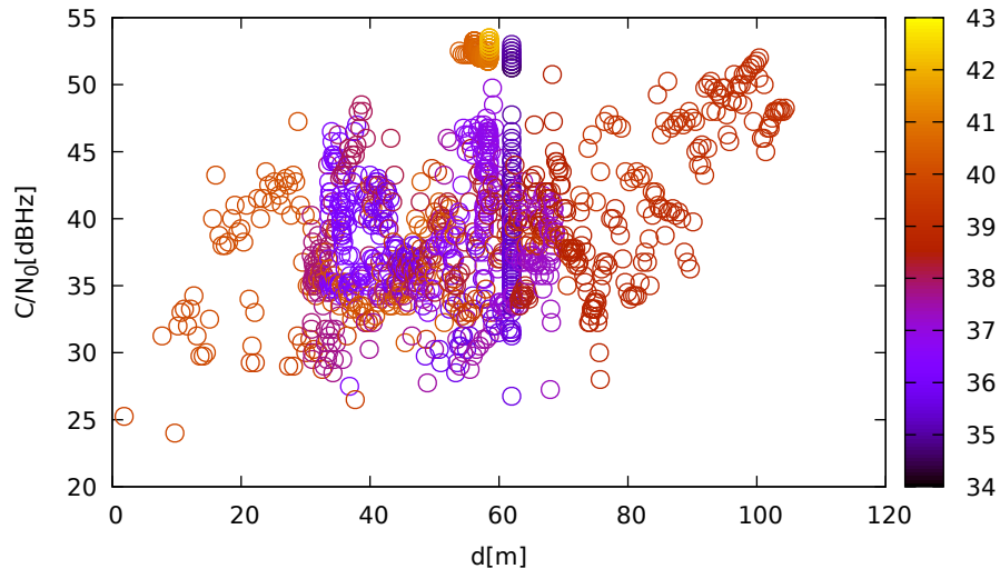
C/N 0 vs distance (LeicaGS18 at C 1 for G32 at L1)
