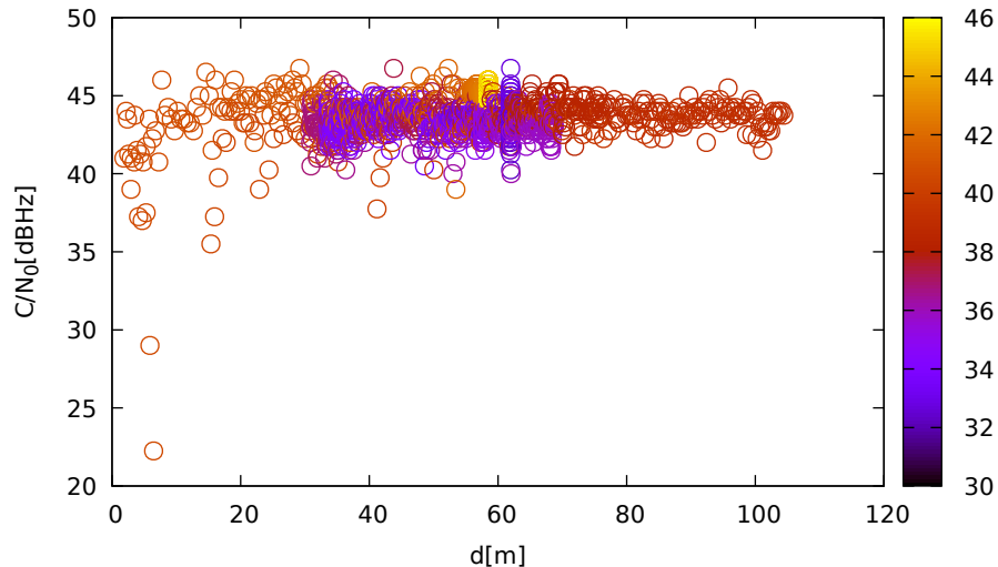
C/N 0 vs distance (LeicaGS18 at C 1 for R06 at L1)
