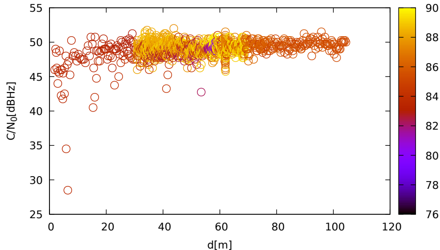
C/N 0 vs distance (LeicaGS18 at C 1 for R07 at L1)
