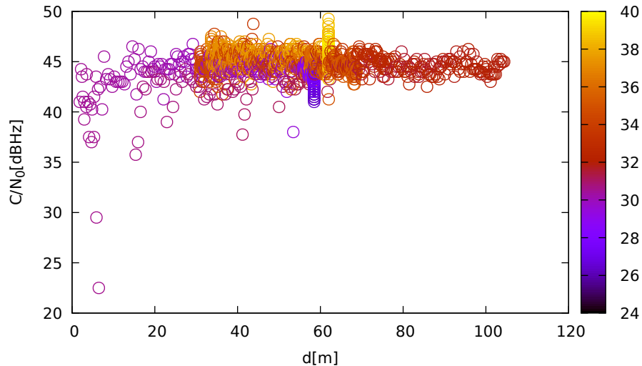
C/N 0 vs distance (LeicaGS18 at C 1 for R08 at L1)
