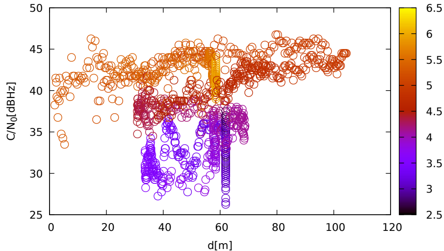
C/N 0 vs distance (LeicaGS18 at C 1 for R14 at L1)
