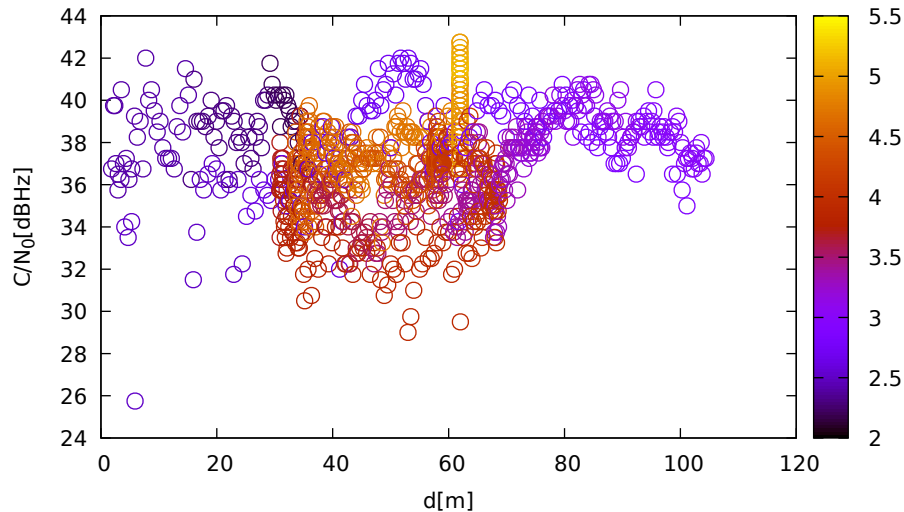
C/N 0 vs distance (LeicaGS18 at C 1 for R15 at L1)
