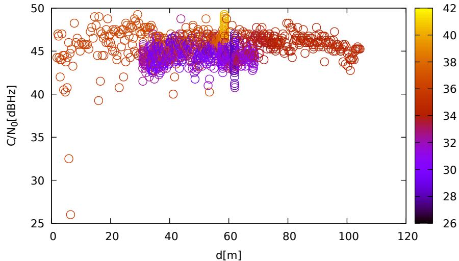
C/N 0 vs distance (LeicaGS18 at C 1 for R21 at L1)
