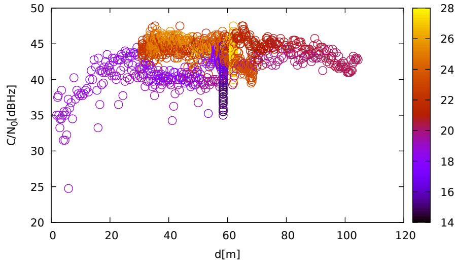
C/N 0 vs distance (LeicaGS18 at C 1 for R23 at L1)
