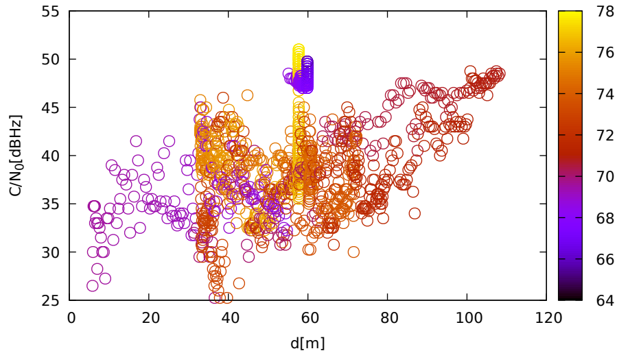
C/N 0 vs distance (TrimbleR8s at C 1 for G01 at L1)
