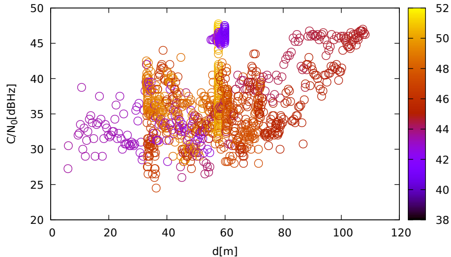
C/N 0 vs distance (TrimbleR8s at C 1 for G03 at L1)
