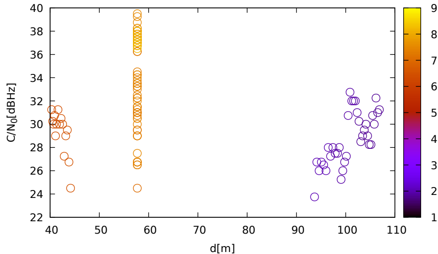
C/N 0 vs distance (TrimbleR8s at C 1 for G04 at L1)
