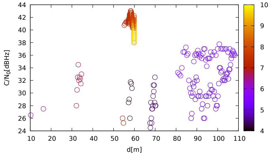
C/N 0 vs distance (TrimbleR8s at C 1 for G10 at L1)
