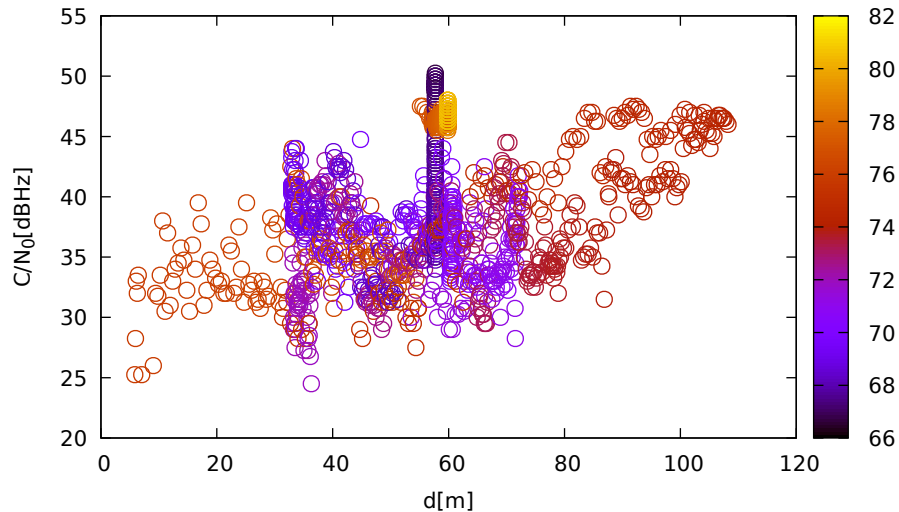
C/N 0 vs distance (TrimbleR8s at C 1 for G11 at L1)
