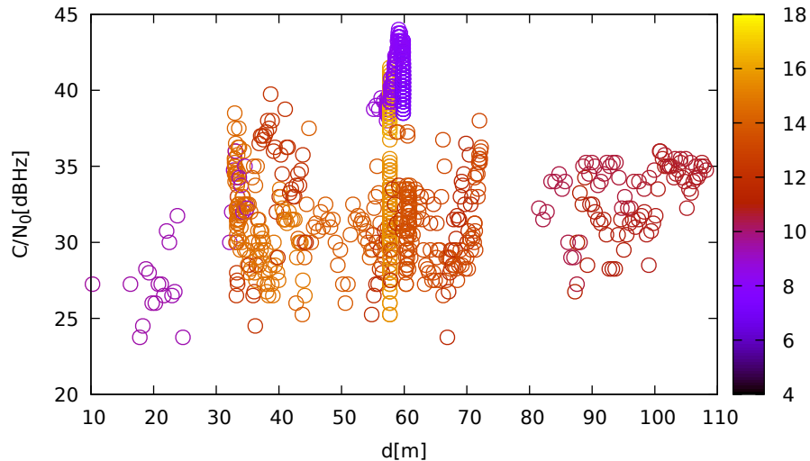
C/N 0 vs distance (TrimbleR8s at C 1 for G17 at L1)
