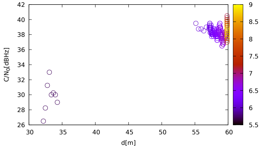
C/N 0 vs distance (TrimbleR8s at C 1 for G21 at L1)
