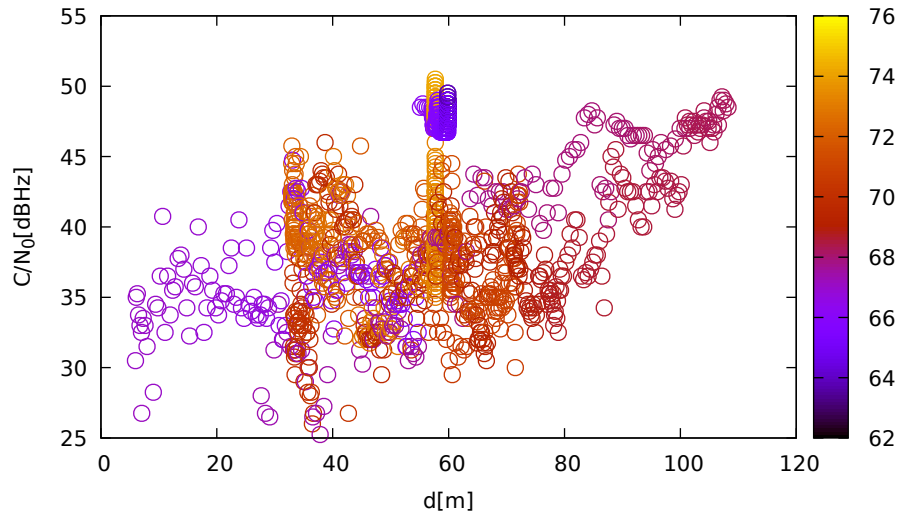
C/N 0 vs distance (TrimbleR8s at C 1 for G22 at L1)
