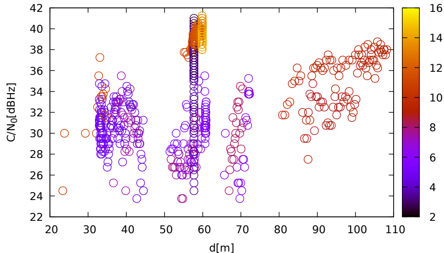
C/N 0 vs distance (TrimbleR8s at C 1 for G27 at L1)
