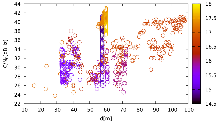
C/N 0 vs distance (TrimbleR8s at C 1 for G28 at L1)
