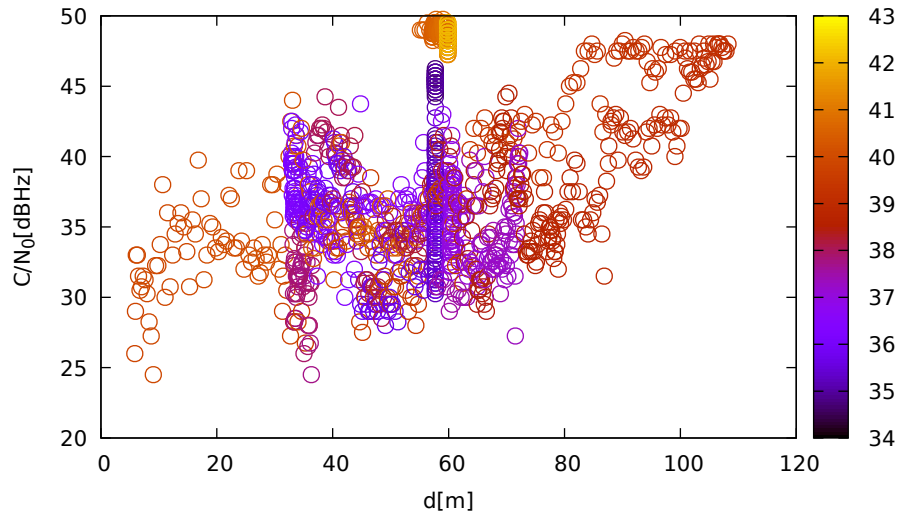
C/N 0 vs distance (TrimbleR8s at C 1 for G32 at L1)
