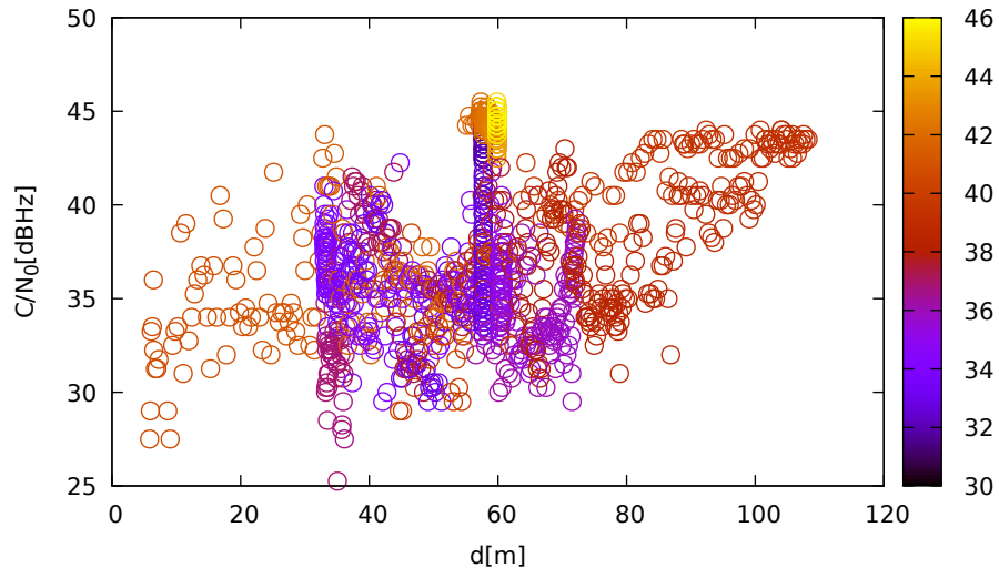
C/N 0 vs distance (TrimbleR8s at C 1 for R06 at L1)
