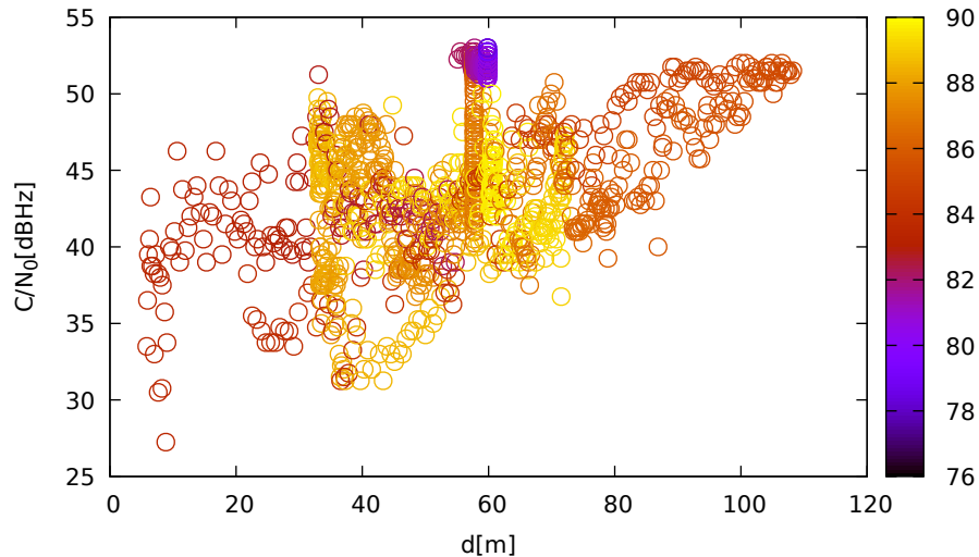
C/N 0 vs distance (TrimbleR8s at C 1 for R07 at L1)
