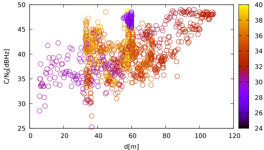
C/N 0 vs distance (TrimbleR8s at C 1 for R08 at L1)
