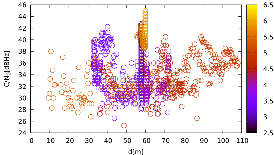
C/N 0 vs distance (TrimbleR8s at C 1 for R14 at L1)
