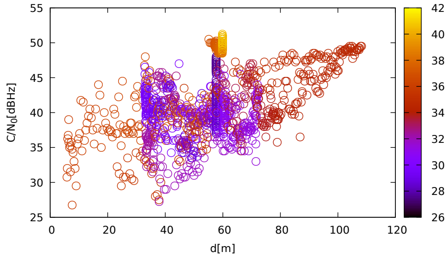
C/N 0 vs distance (TrimbleR8s at C 1 for R21 at L1)
