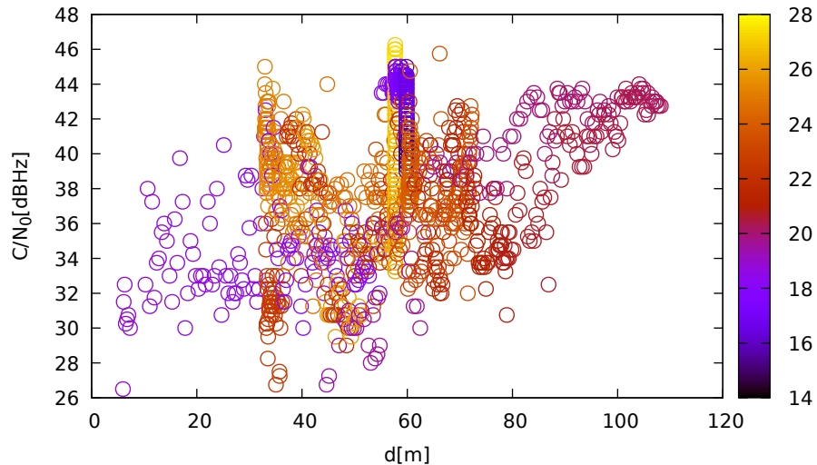
C/N 0 vs distance (TrimbleR8s at C 1 for R23 at L1)
