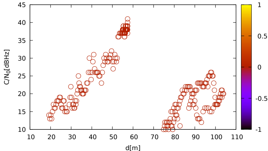
C/N 0 vs distance (ublox9 at C 1 for E02 at L1)
