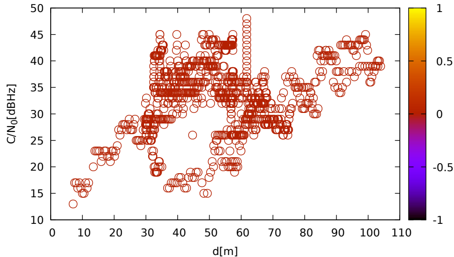
C/N 0 vs distance (ublox9 at C 1 for E04 at L1)
