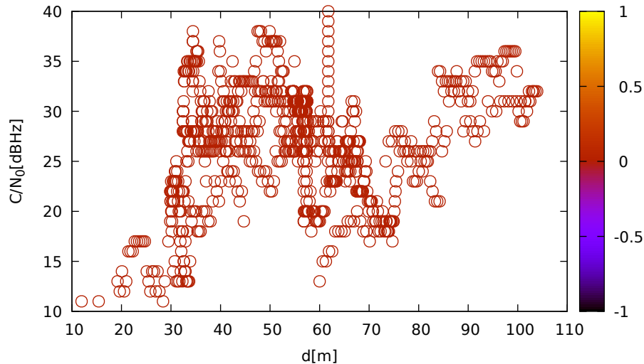
C/N 0 vs distance (ublox9 at C 1 for E05 at L1)
