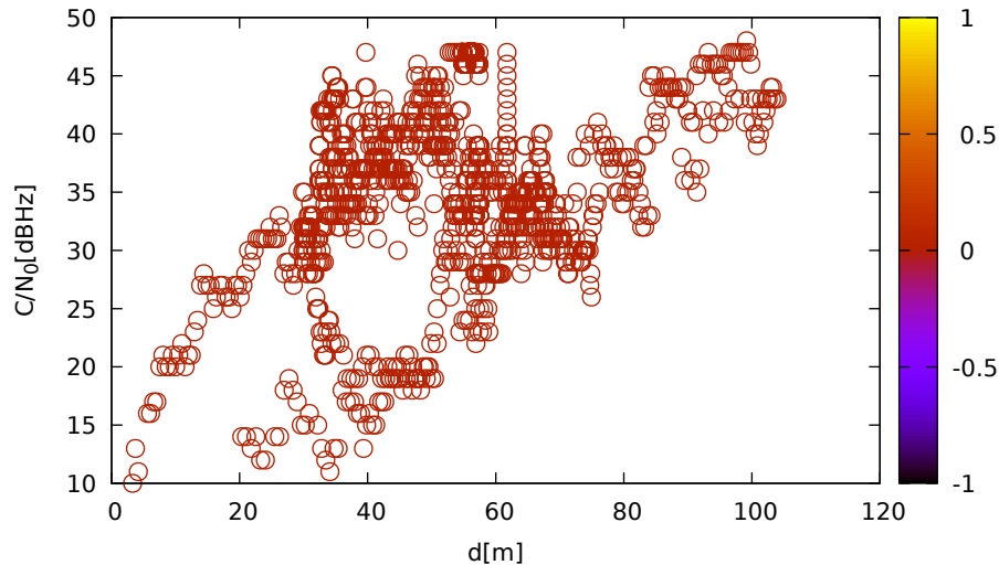
C/N 0 vs distance (ublox9 at C 1 for E09 at L1)
