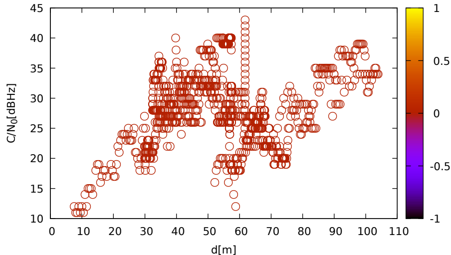
C/N 0 vs distance (ublox9 at C 1 for E11 at L1)
