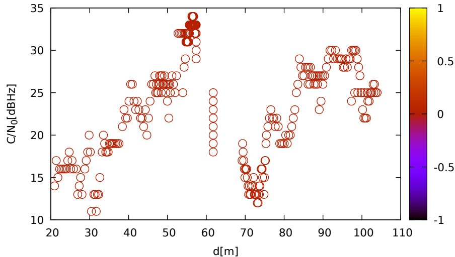
C/N 0 vs distance (ublox9 at C 1 for E12 at L1)
