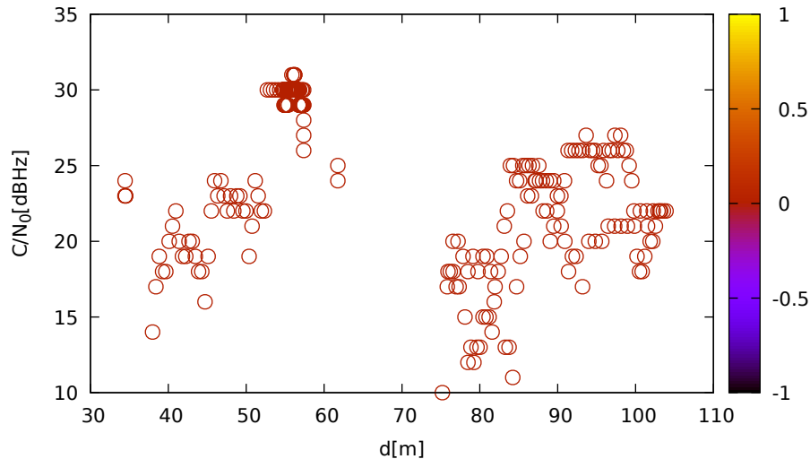
C/N 0 vs distance (ublox9 at C 1 for E19 at L1)
