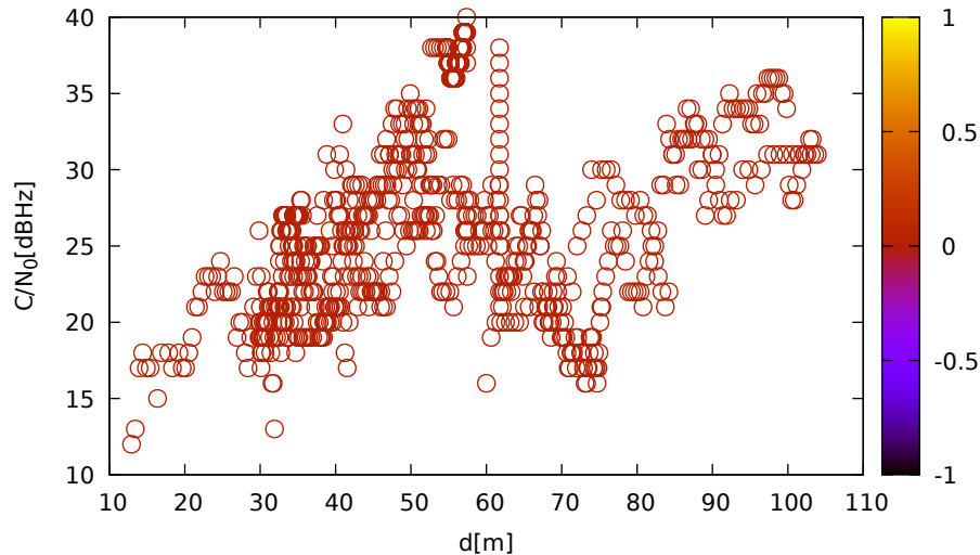
C/N 0 vs distance (ublox9 at C 1 for E30 at L1)
