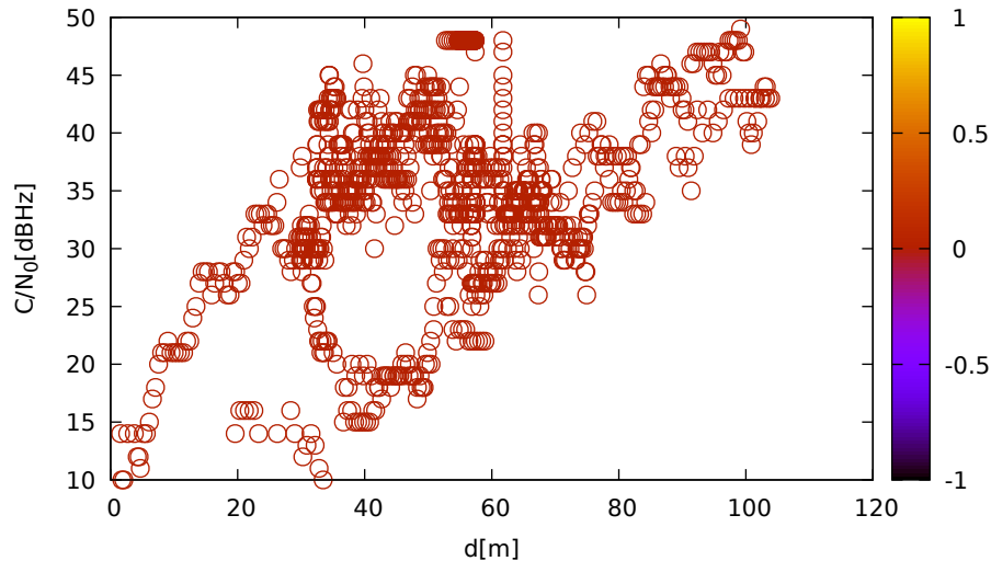
C/N 0 vs distance (ublox9 at C 1 for E36 at L1)
