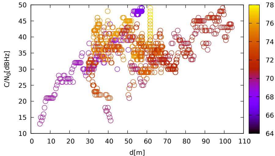
C/N 0 vs distance (ublox9 at C 1 for G01 at L1)
