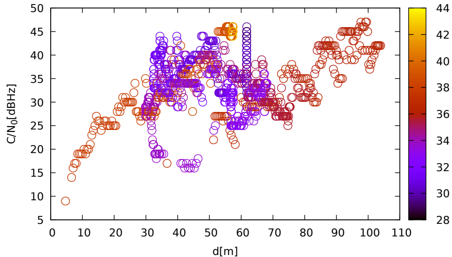
C/N_0 vs distance (ublox9 at C_1 for G08 at L1)
