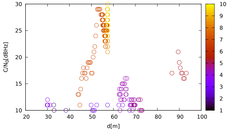
C/N_0 vs distance (ublox9 at C_1 for G10 at L1)
