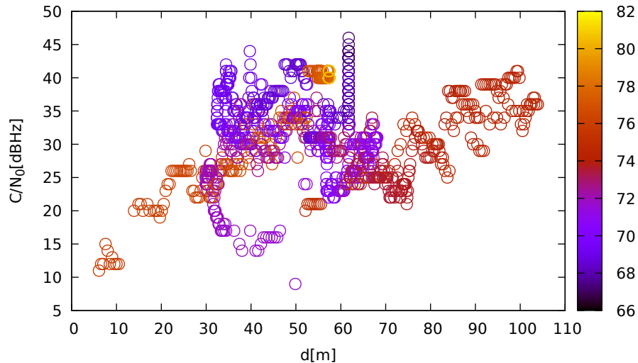
C/N 0 vs distance (ublox9 at C 1 for G11 at L1)
